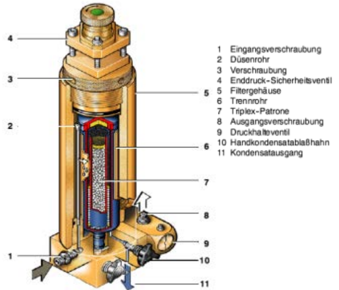
Filtersystem P 21
